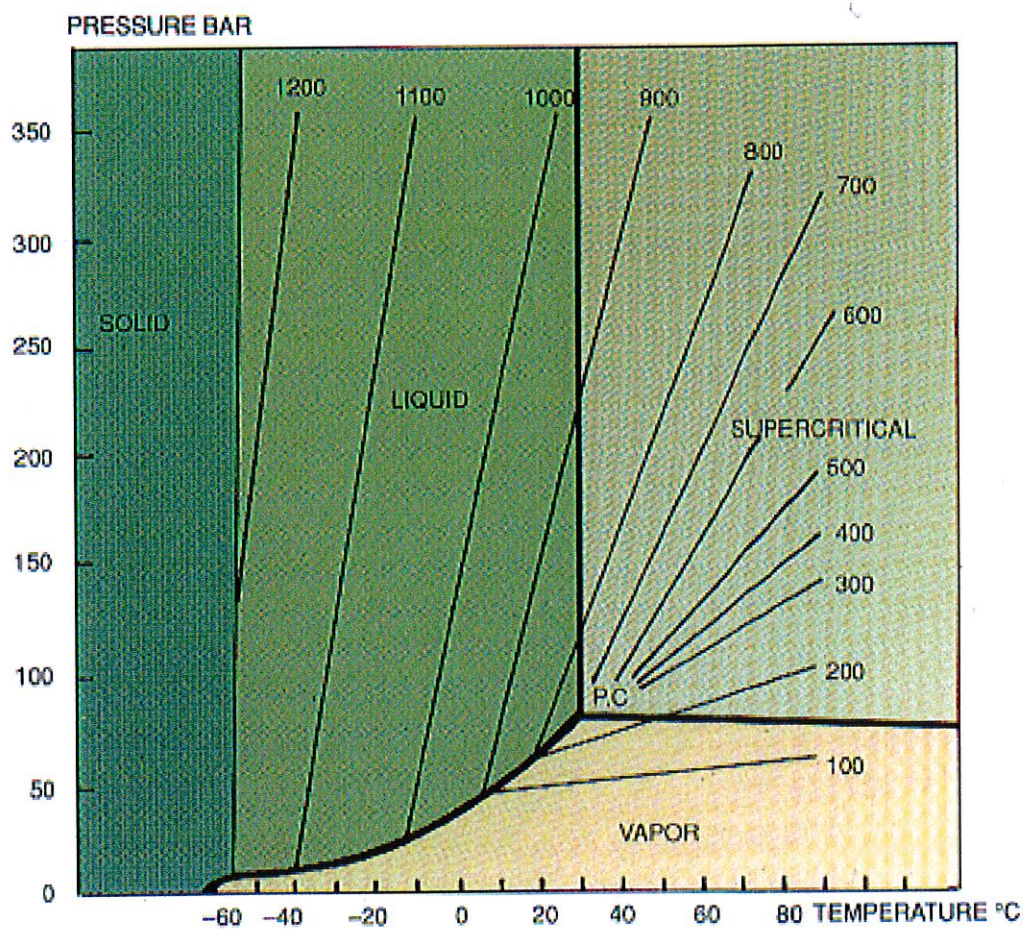
Phase diagram of CO 2 . Constant density lines (g/l)
